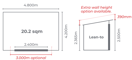
Havelock 4.8m x 4.2m DLL4842 Havelock Extra Height DLLEH4842
