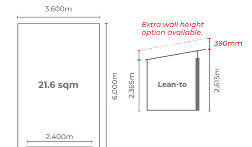
Wairarapa 3.6m x 6m DLL3660 Wairarapa Extra Height DLLEH3660
