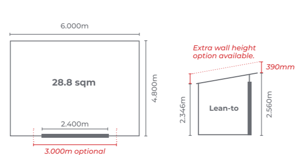
Oxford 6m x 4.8m DLL6048 Oxford Extra Height DLLEH6048
