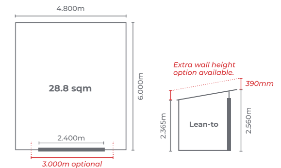
Paihia 4.8m x 6m DLL4860 Paihia Extra Height DLLEH4860
