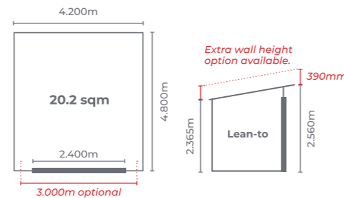
Glenburn 4.2m x 4.8m DLL4248 Glenburn Extra Height DLLEH4248
