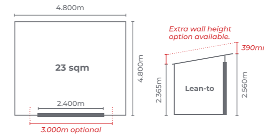
Ardmore 4.8m x 4.8m DLL4848 Ardmore Extra Height DLLEH4848
