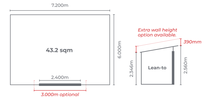
Cromwell 7.2m x 6m DLL7260 Cromwell Extra Height DLLEH7260
