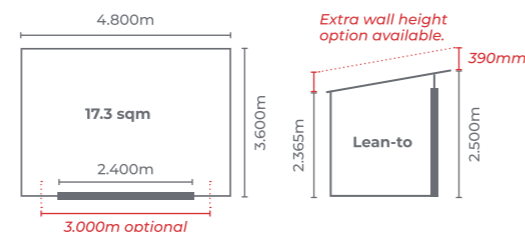
Whitford 4.8m x 3.6m DLL4836 Whitford Extra Height DLLEH4836
