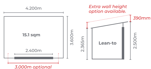
Waiheke 4.2m x 3.6m DLL4236 Waiheke Extra Height DLLEH4236
